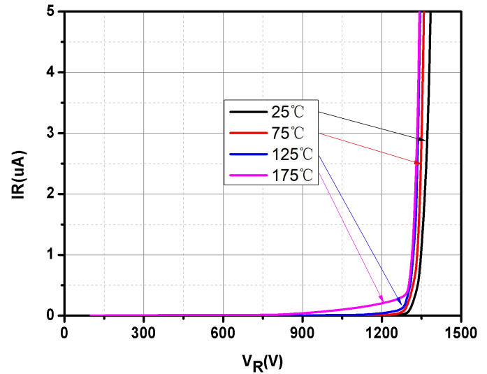
Fig.2-Typical Reverse Characteristics
