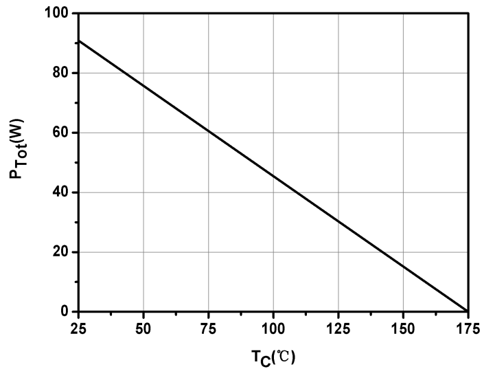
Fig.6-Power Derating
