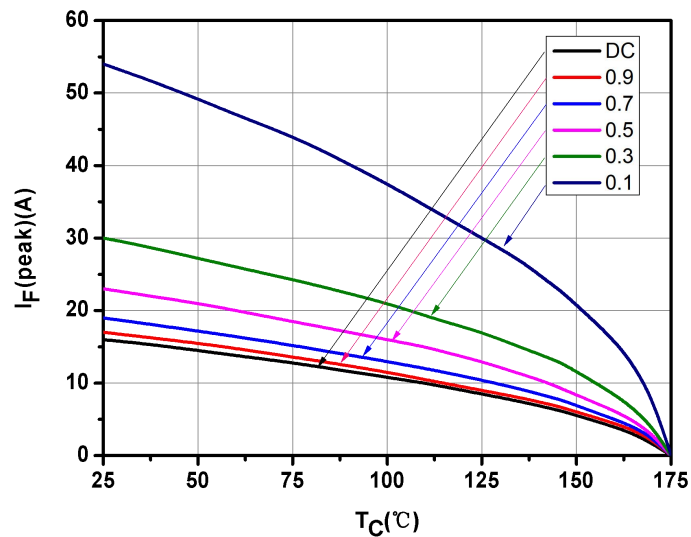
Fig.7-Current Derating
